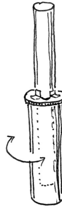
narrow straw, washer, tape, wide straw
